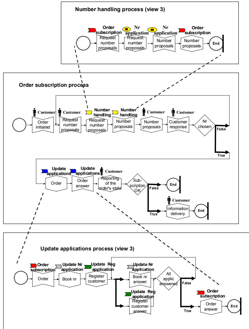
Fig. 10. Some of the process diagrams in view 3.
