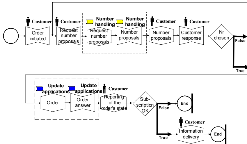
Fig. 9. The Order subscription process (view 2).
