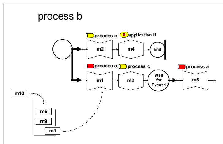
Fig. 4. A process instance with the input queue.
