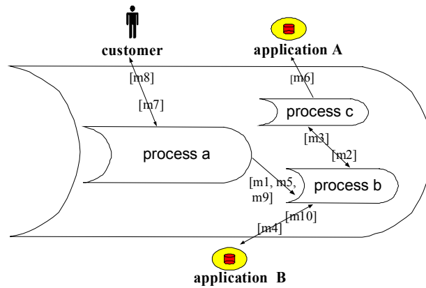
Fig. 3. The static diagram in BML visualises the structure of the processes in a system.
