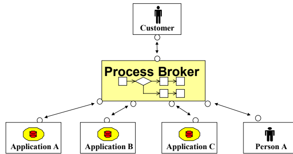
Fig. 6. The customer does not communicate directly with the applications and other people, but only through the Process Broker.
