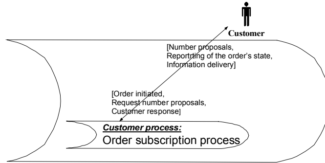
Fig. 7. The static diagram in view 1
