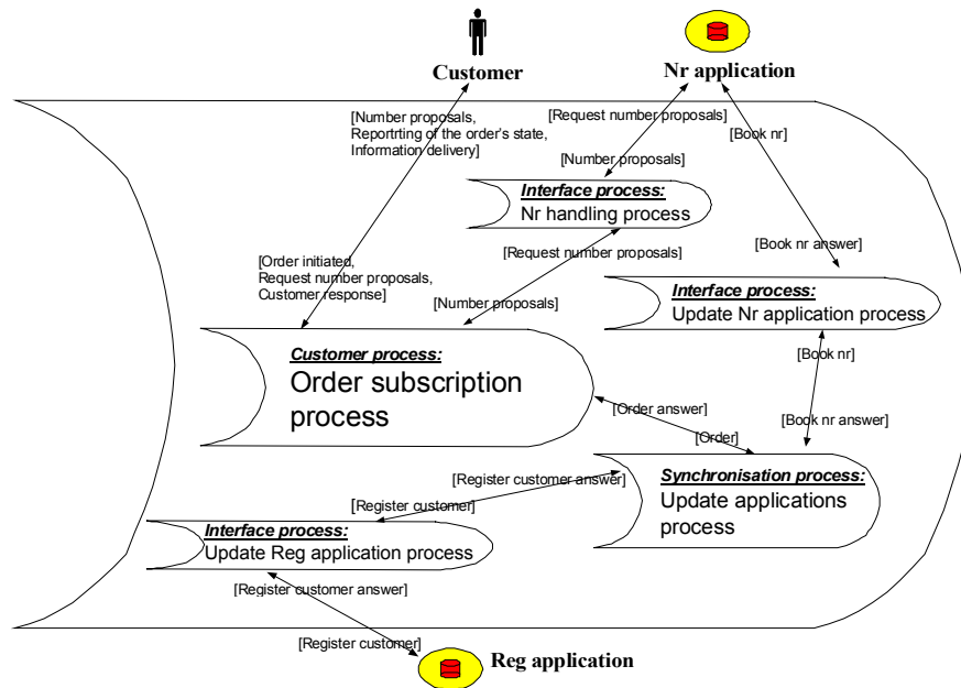
Fig. 11. The static diagram in view 3.
