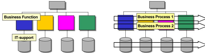
Fig. 1. The traditional function oriented structure, to the left, with the “stovepipe” like relation between business functions and IT systems. To the right the process oriented organisation which requires an integration of the IT systems.
