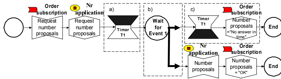
Fig. 12. The Number handling process (view 4).
