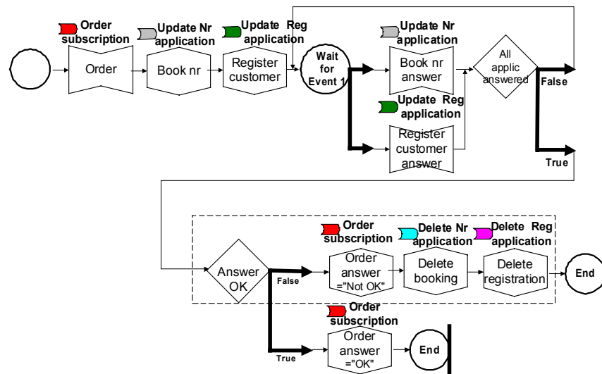
Fig. 13. The Update application process (view 5).
