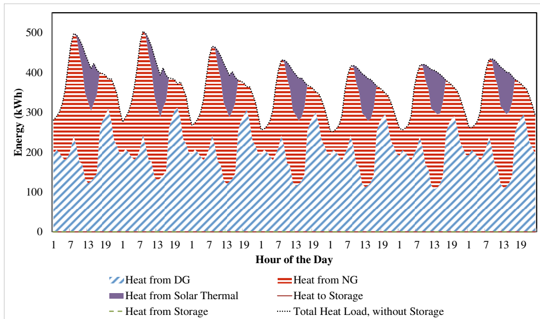
Figure 6. Forecasted heat demand and CO 2 minimizing operation schedule for the S3 case and the week from Sunday 09-Jan-11 to Sunday 16-Jan-11
