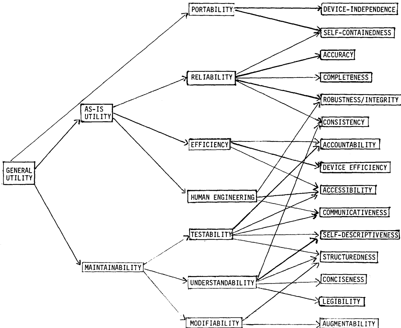
Fig. 1 - Software Quality Characteristics Tree
