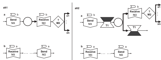
Figure 9: Request/Reply
