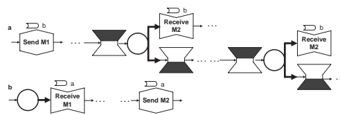
Figure 10: Synchronous Polling
