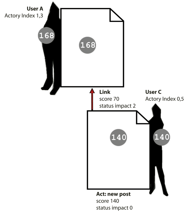
Figure 4. Distribution of score between actors and activities when creating a post.
