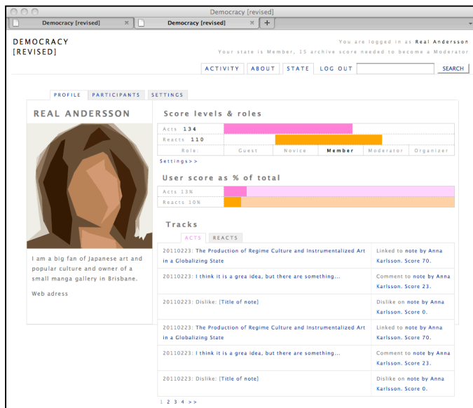
Figure 1. Web based prototype built in Drupal visualizing user state.
