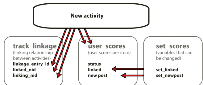
Figure 5. The scoring system in Drupal when creating an activity.
