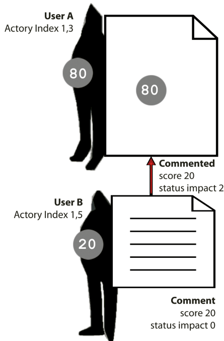
Figure 3. The distribution of score between users and activities when a user comments a post.
